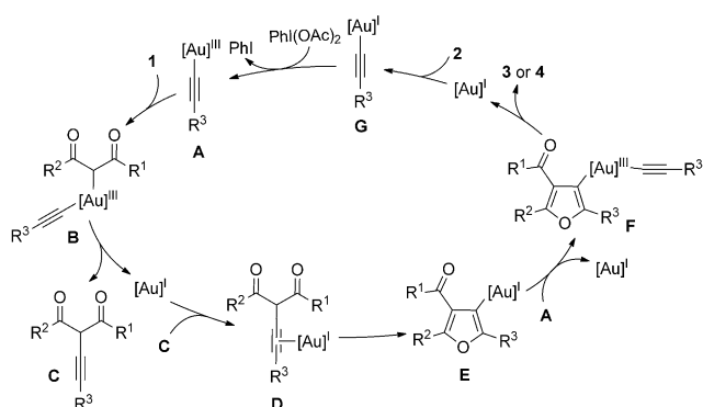
Scheme 3. Proposed mechanism.
